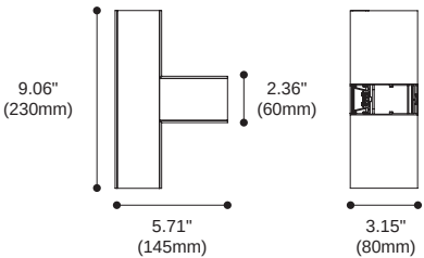
T Type
