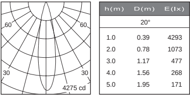
2117.423-V
