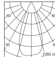
2117.437-V
