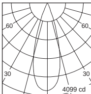
2117.437-V
