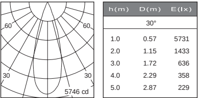
2117.460-V
